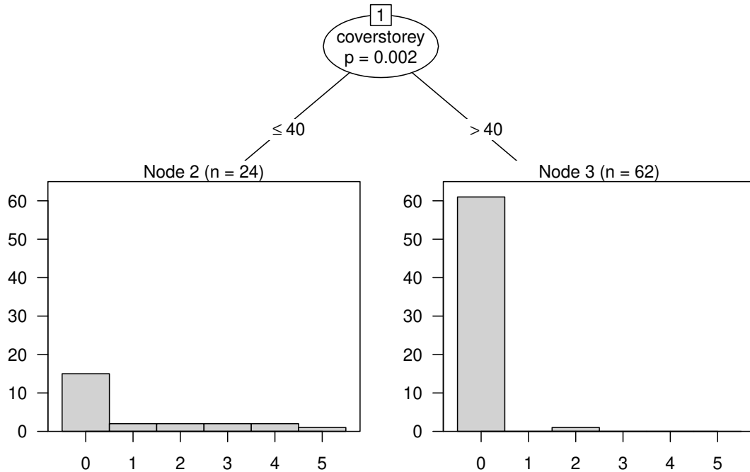
Figure 2: Conditional regression tree for the tree pitip data.
